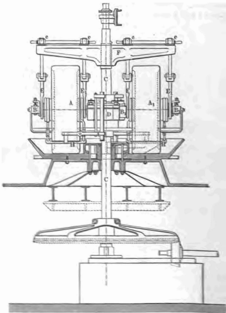
FIG. 9. — Vertical Engine
