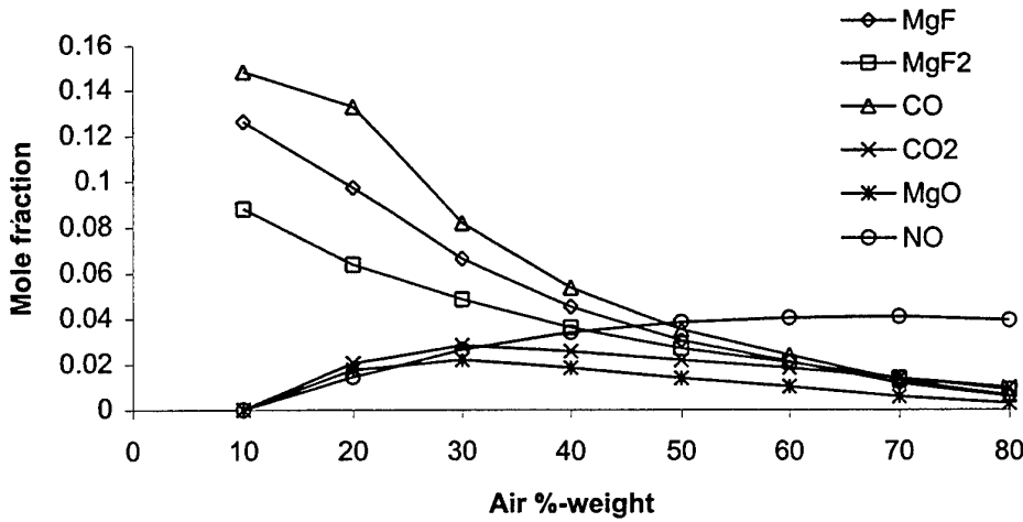
Figure 14: Concentration profiles of major species from MTV-1 products reacting with air.
