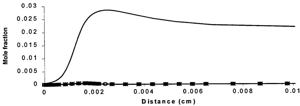
Figure 33: Profiles of CF (top) and CF 2 (bottom) species against distance from burner's exit plane. Mixtures: ___stoichiometric, -* UK Flare, -o US igniter..
