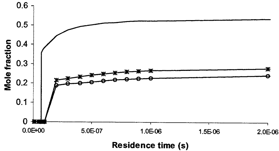
Figure 28: Distribution of MgF_2 against residence time. MT compositions: ___stoichiometric, -* UK Flare, -o- US igniter.
