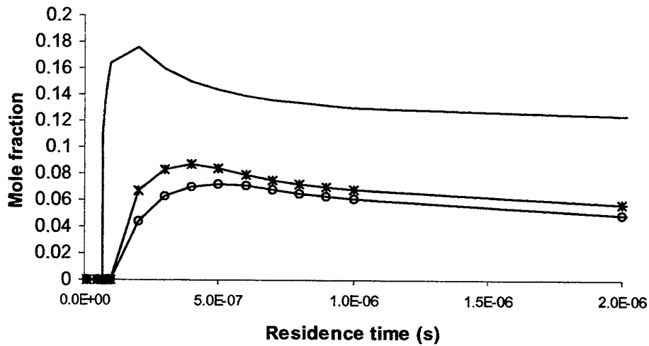
Figure 29: Profiles of CF against residence time. MT compositions: ___stoichiometric, -* UK Flare, -o- US igniter.
