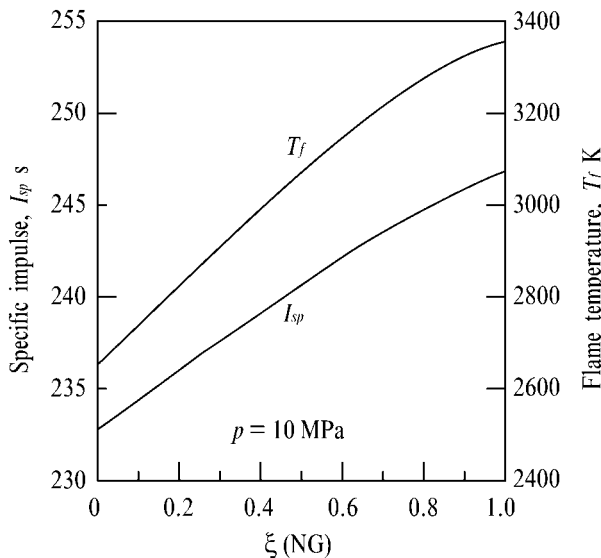
Figure 4-3. Specific impulse and adiabatic flame temperature of NC-NG double-base propellant as a function of the mass fraction of NG.
