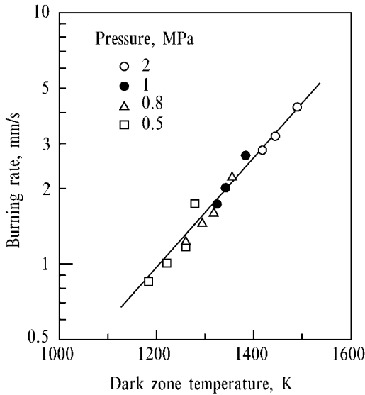
Figure 7-40. Burning rate versus dark zone temperature of HMX-CMDB propellant at different pressures.
