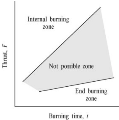
Figure 9-2. Zones of burning in rocket motor.
